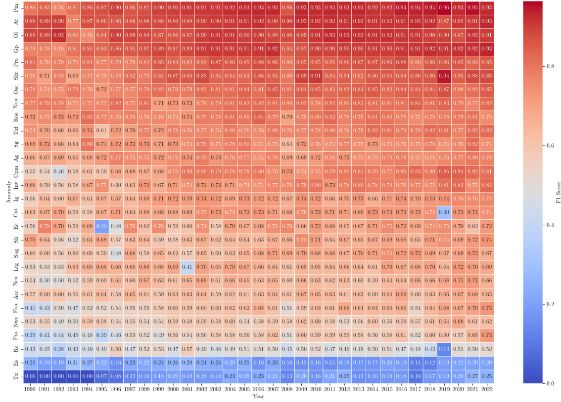
Figure A2. Heatmap of Machine Learning Model Quality by Year - F1 Scores The heatmap shows F1 Scores by anomaly and by year using the Machine Learning model. The F1 Score measures a model's accuracy while considering both the precision (the proportion of true positive predictions among all positive predictions) and recall (the proportion of true positive predictions among all actual positive cases) of the predictions, providing a single metric for the test's accuracy. A higher F1 Score indicates that a model for a given anomaly and year has a balance of high precision (few false positives) and high recall (few false negatives).
