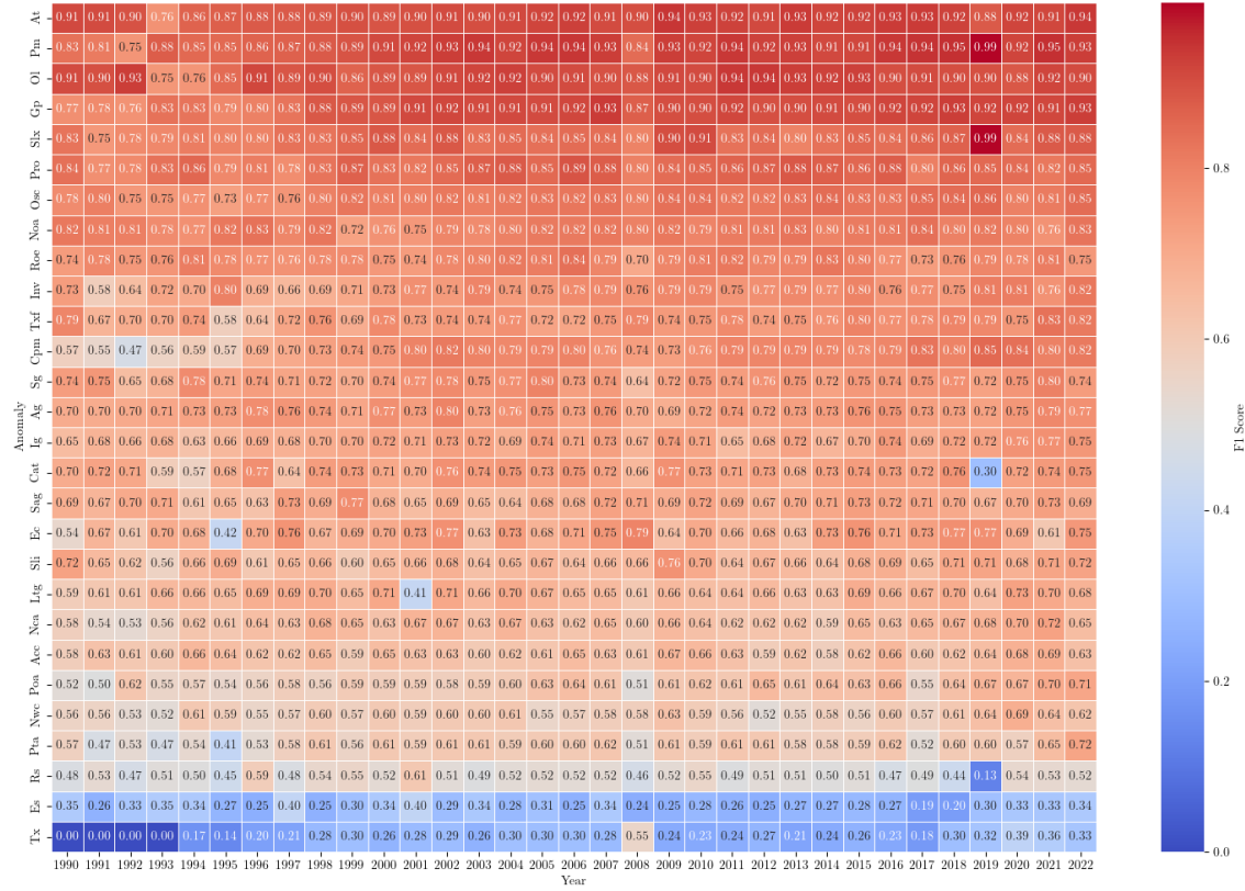
Figure 4. Heatmap of Martingale Model Quality by Year - F1 Scores The heatmap shows F1 Scores by anomaly and by year using the Martingale model. The F1 Score measures a model's accuracy while considering both the precision (the proportion of true positive predictions among all positive predictions) and recall (the proportion of true positive predictions among all actual positive cases) of the predictions, providing a single metric for the test's accuracy. A higher F1 Score indicates that a model for a given anomaly and year has a balance of high precision (few false positives) and high recall (few false negatives).
