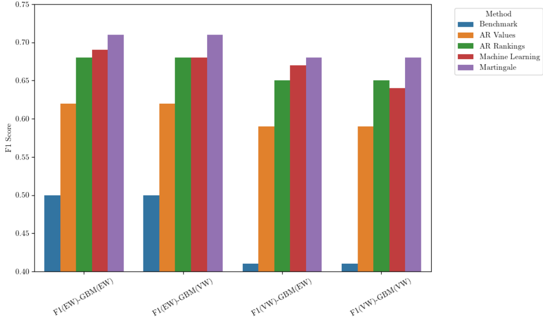
(a) F1 Scores for All Models
