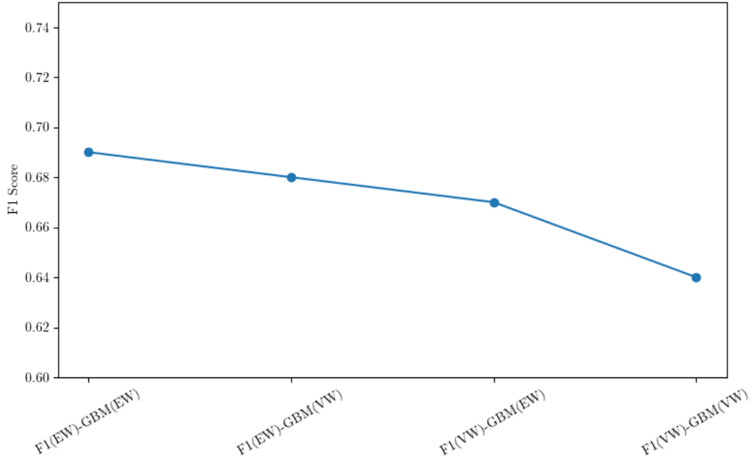
(b) F1 Scores for Machine Learning Model
