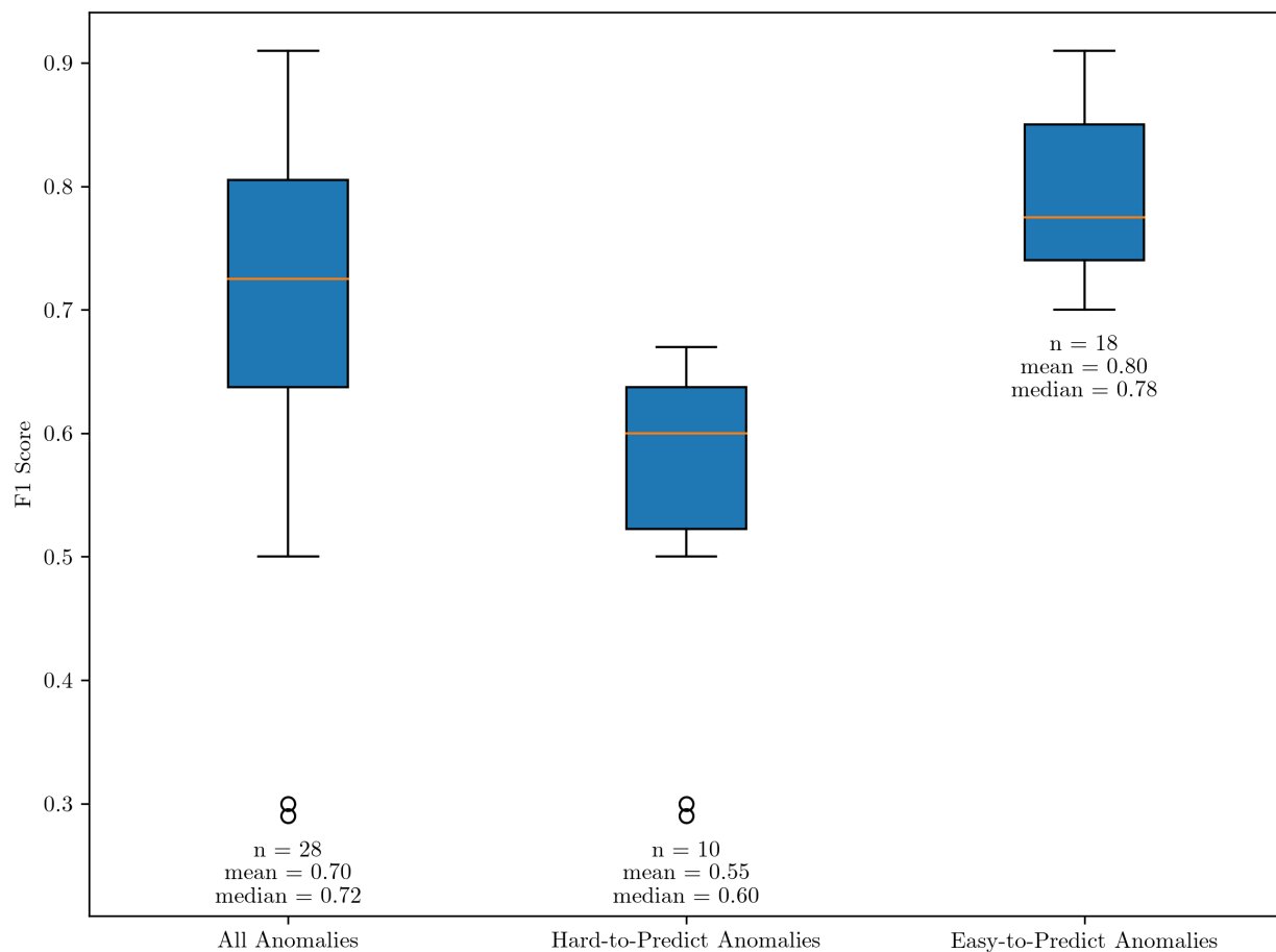
Figure 10. Boxplot of F1 Scores by Anomaly Group
